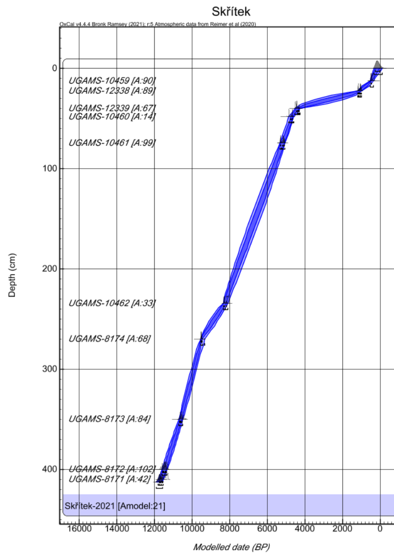
Supplementary Material, Fig. S1 – Depth-age models of four profiles from the Jeseníky Mts.
