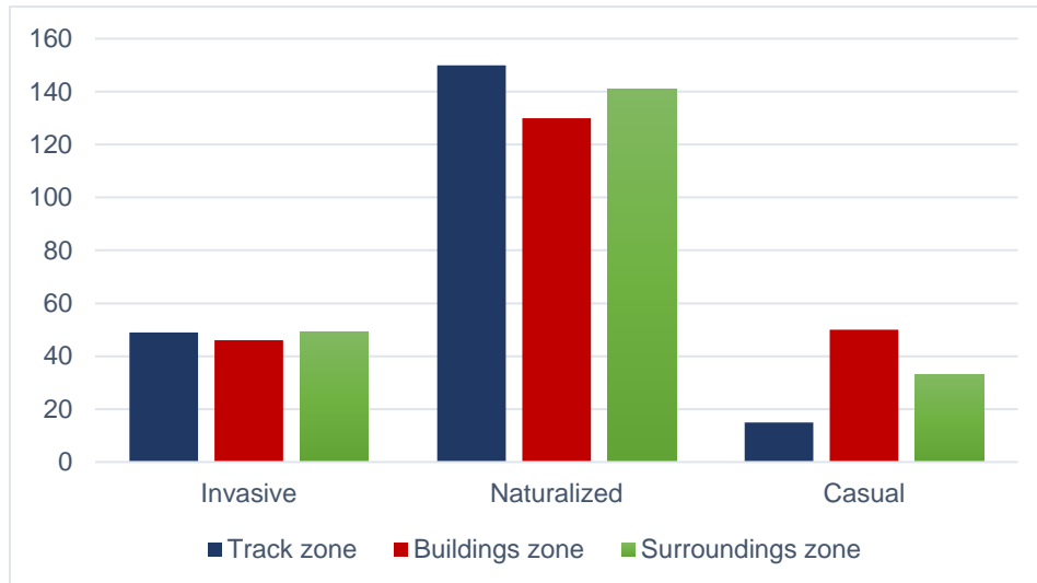
Supplementary Fig. S1. (A) The number of aliens in examined zones
