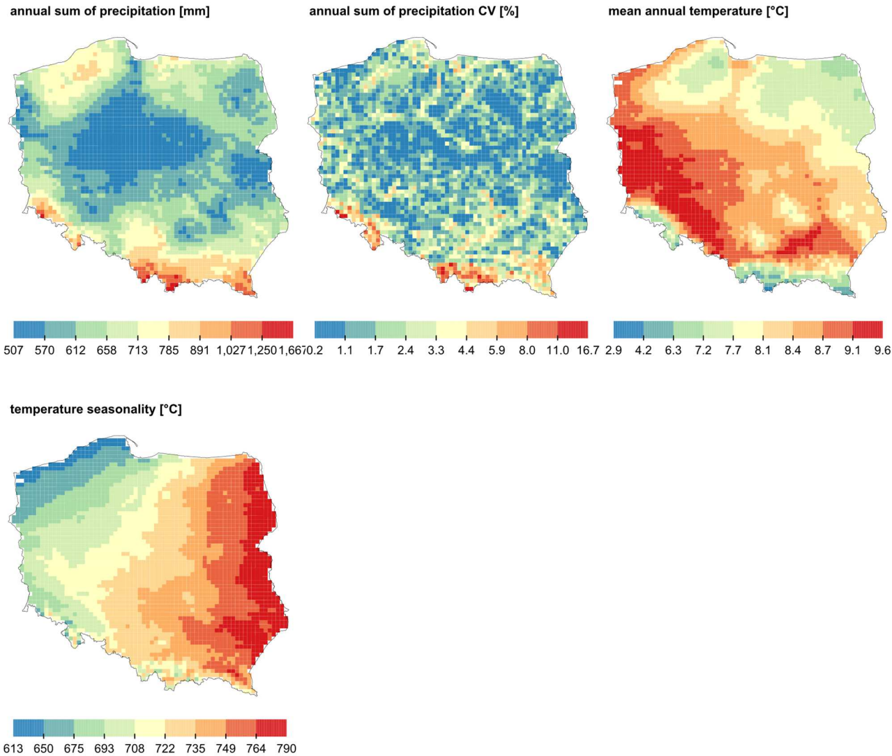
Supplementary Fig. S3. Spatial distribution of explanatory variables representing climate included in the final models. The maps were produced using the Fisher method.
