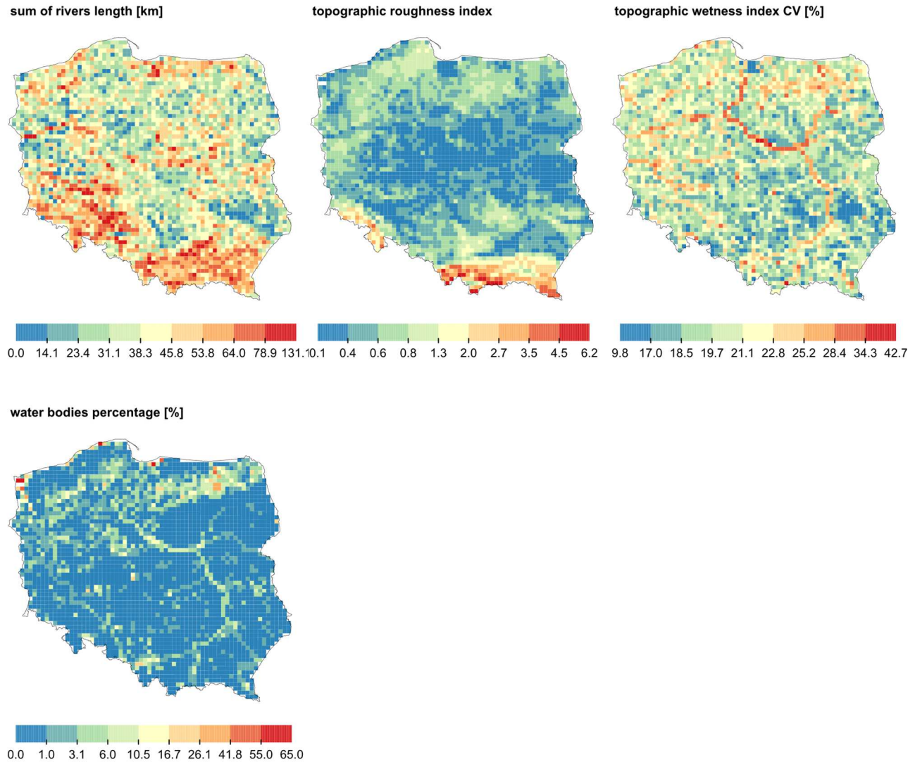
Supplementary Fig. S5. Spatial distribution of topographic explanatory variables included in the final models. The maps were produced using the Fisher method.
