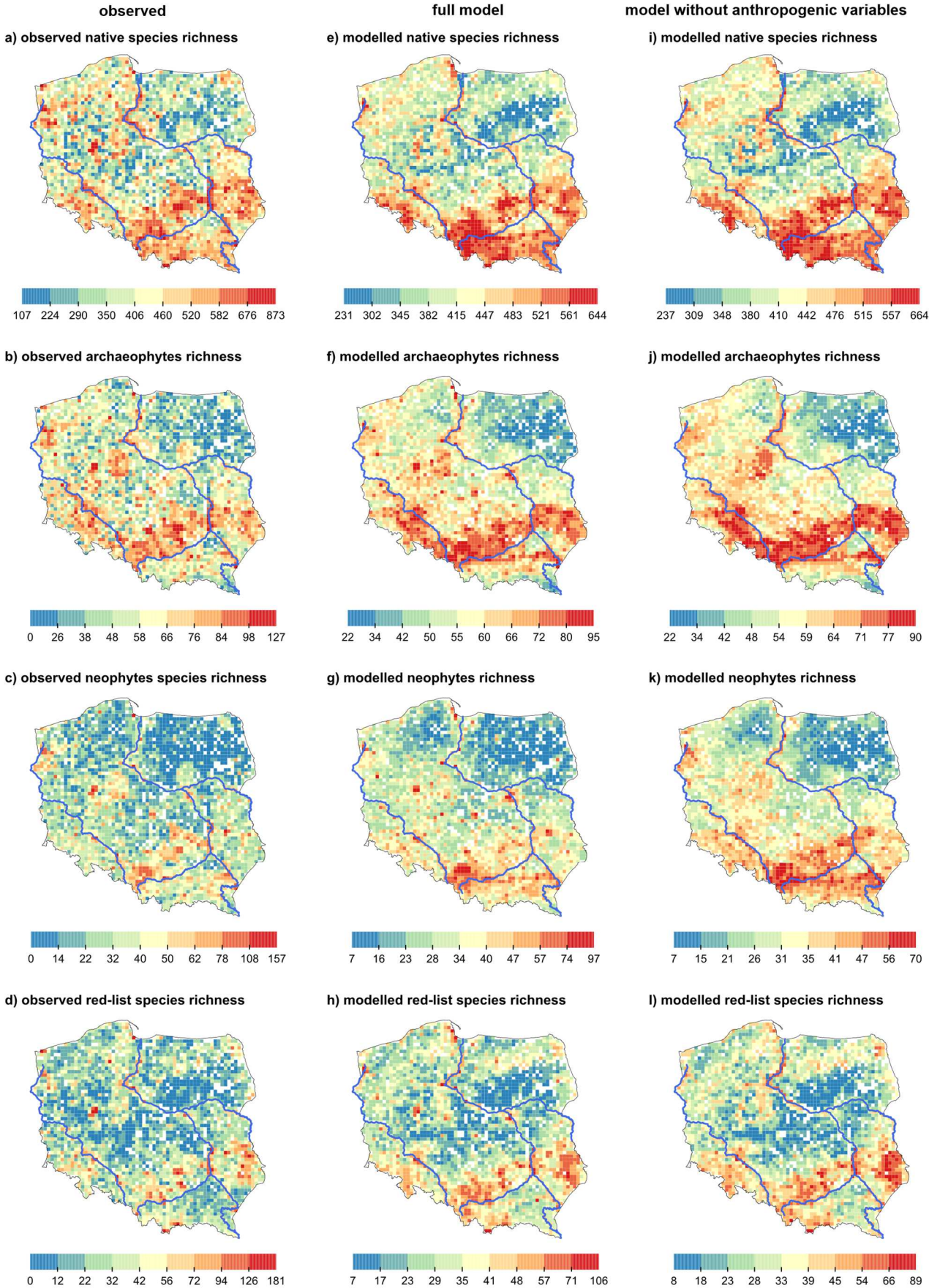
Supplementary Fig. S7. Spatial distribution of observed (first column) and predicted (second and third columns) species richness (SR) for native species (first row), archaeophytes (second row), neophytes (third row), and red-list species (fourth row). The results for the full model are in the middle column, while the model without anthropogenic variables is in the third column. The white areas denote unsampled squares.
