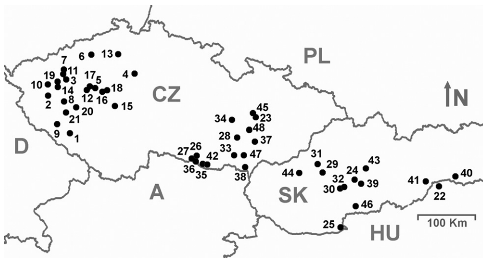
Fig. 1. – Map of Central Europe showing the localities sampled (numbered black circles). Abbreviations: A – Austria, CZ – Czech Republic, D – Germany, HU – Hungary, PL – Poland, SK – Slovakia. For detailed characteristics of each locality see Svoboda et al. (2010).
