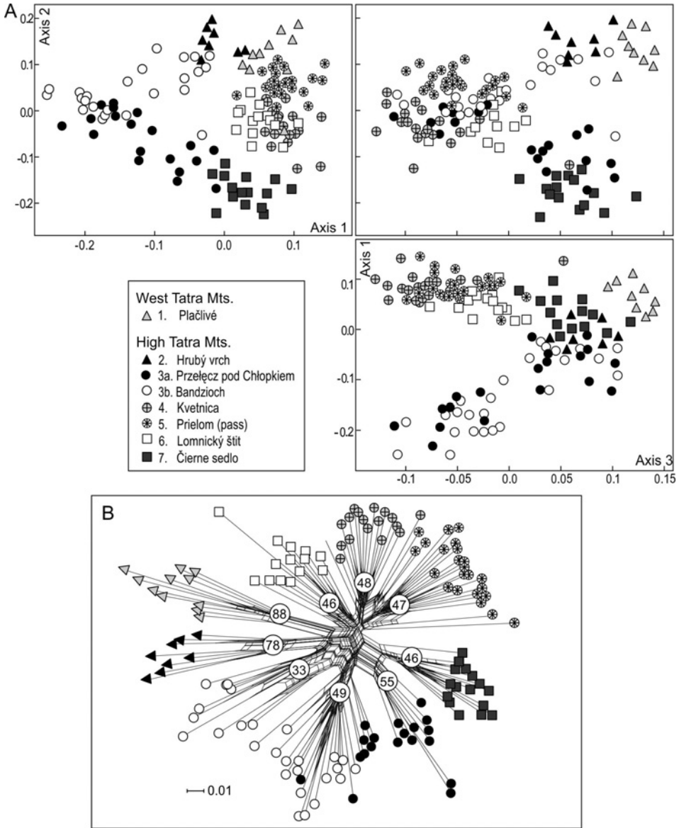
Fig. 3. – Analysis of Cochlearia tatrae based on 208 AFLP fragments of the 133 individuals studied. (A) Principal Coordinate Analysis diagram based on Jaccard’s coefficient: ordination at 1 vs. 2, 1 vs. 3 and 2 vs. 3 axes. (B) Neighbour-Net network based on Nei and Li’s (1979) genetic distances. Numbers along the branches are bootstrap values based on 10^5 replicates.
