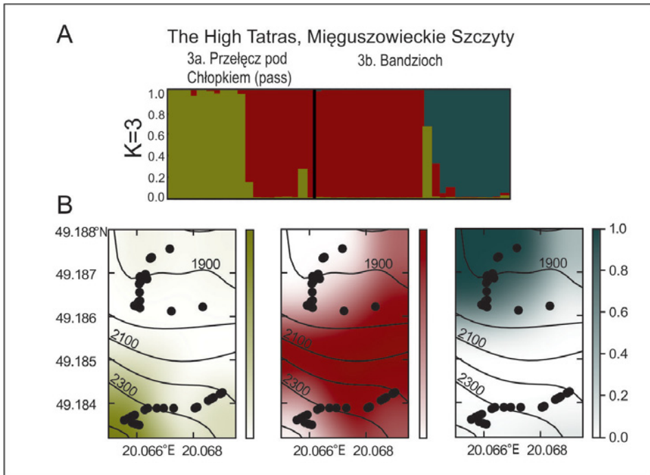
Fig. 2. – Bayesian clustering of Cochlearia tatrae individuals from the Mięguszwieckie Szczyty massif (populations no. 3a and 3b) using TESS, based on AFLP data ( K = 3 ). (A) Bar plot of 44 individuals analysed. (B) Extrapolated probability distribution of the membership of particular geographical space for the three groups based on the Bayesian analysis (colours correspond to those in A); location of genotyped individuals is indicated by black circles.
