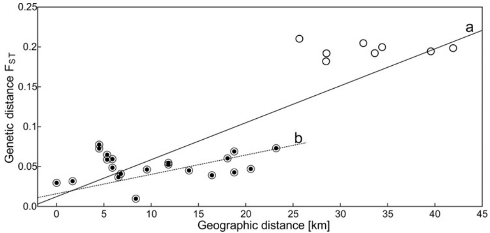
Fig. 4. – Scatterplot showing the results of the Mantel test of the similarity of the matrix of genetic distances (pairwise F_{ST} ) and that of geographic distances (km), supporting the IBD model. Only the lines that fit (a) all populations of Cochlearia tatrae and (b) populations from the High Tatra Mts are shown.
