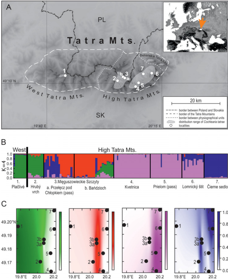
Fig. 1. – Distribution and genetic structure of Cochlearia tatrae in the Tatra Mts. (A) Sampled populations (white circles, numbers refer to the number assigned to each of the populations in Table 1), distribution of C. tatrae (light grey areas), borders of the Tatra Mts and its internal units (white dashed lines). (B) Results of the Bayesian population structure analysis of all individuals of C. tatrae based on AFLP markers, inferred using TESS. Bar graphs of individuals for K = 4 ; populations are separated by vertical lines. (C) Probability distribution of the membership of particular geographical areas for four genetic groups based on the TESS analysis (see text for details; colours correspond to those used in B). Population locations in geographical space are indicated by black circles.
